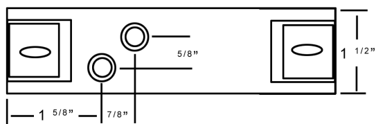
Type OF Offset at 1 end
