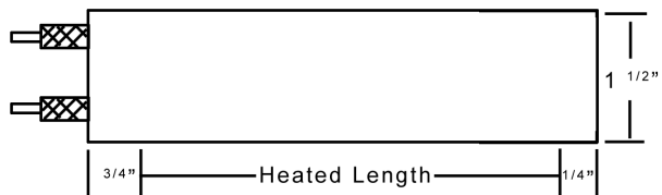
Type SF1 Flexible insulated leads
